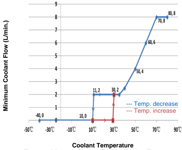
Figure 1: Minimum Coolant Flow vs. Coolant Temperature
