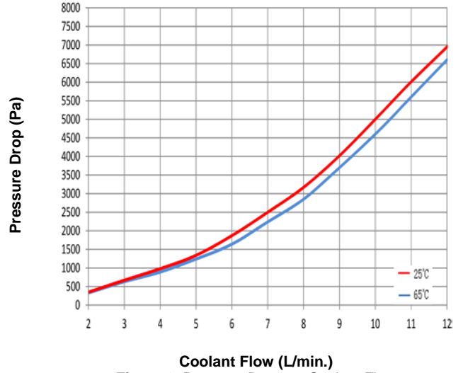
Figure 2: Pressure Drop vs. Coolant Flow
