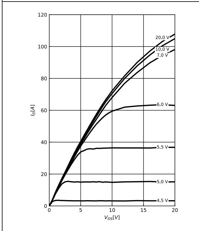
Diagram 3: Typ. output characteristics
