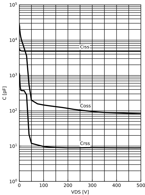
Diagram 11: Typ. capacitances
