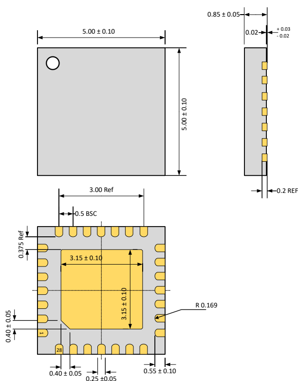
Figure 22: QFN28 5x5mm
