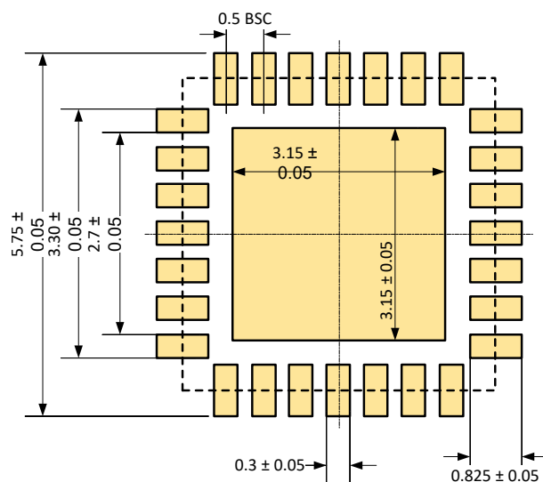
Figure 22: Board layout
