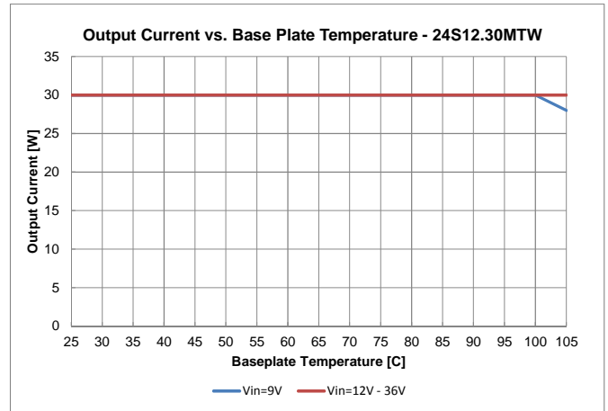
Fig. 11: 24S12.30MTW (ROHS) Derating Curve
