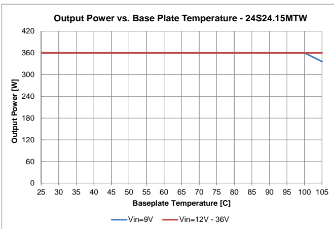
Fig. 12: 24S24.15MTW (ROHS) Derating Curve
