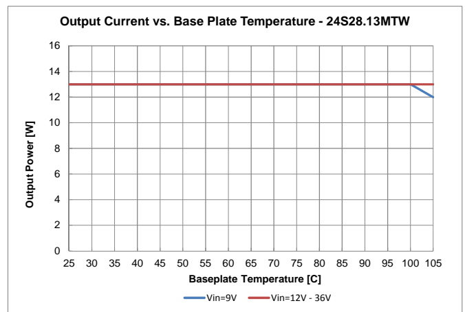
Fig. 15: 24S28.13MTW (ROHS) Derating Curve
