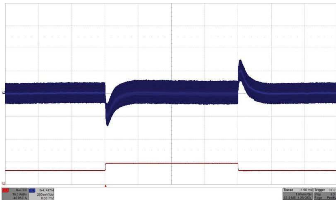
Fig. 30: Output voltage response to load current step change 50% - 75% - 50% ( 6.5A - 9.75A - 6.5A ) with di/dt = 1A/\mu s at V_{IN} = 24V . Top trace (C4): Output voltage (200 mV/div.). Bottom trace (C3): Load current (10A/div.). C_O = 470\mu F/70m\Omega . Time: 1ms/div.
