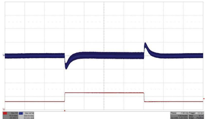
Fig. 31: Output voltage response to load current step change 100% - 50% ( 6.5A - 13A - 6.5A ) with di/dt = 1A/\mu s at V_{IN} = 24V . Top trace (C4): Output voltage (500 mV/div.). Bottom trace (C3): Load current (10A/div.). C_O = 470\mu F/70m\Omega . Time: 1ms/div.
