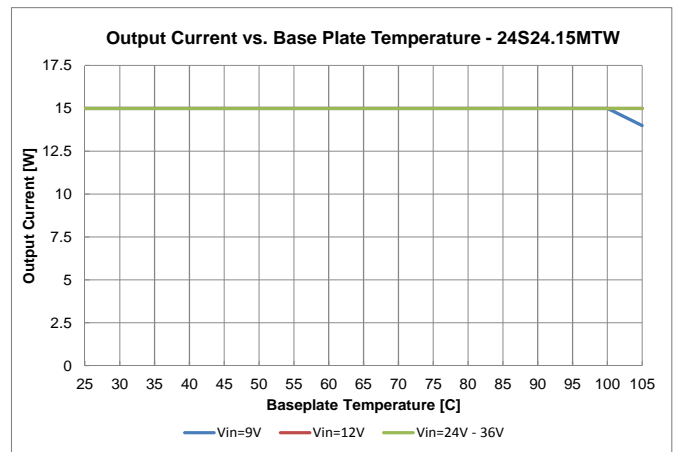
Fig. 13: 24S24.15MTW (ROHS) Derating Curve
